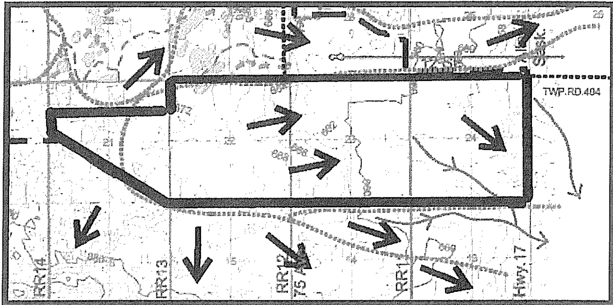
FIGURE 6 - IDP MAP 2 - TOPOGRAPHY/STORM DRAINAGE PATTERNS (SOUTH UE)
