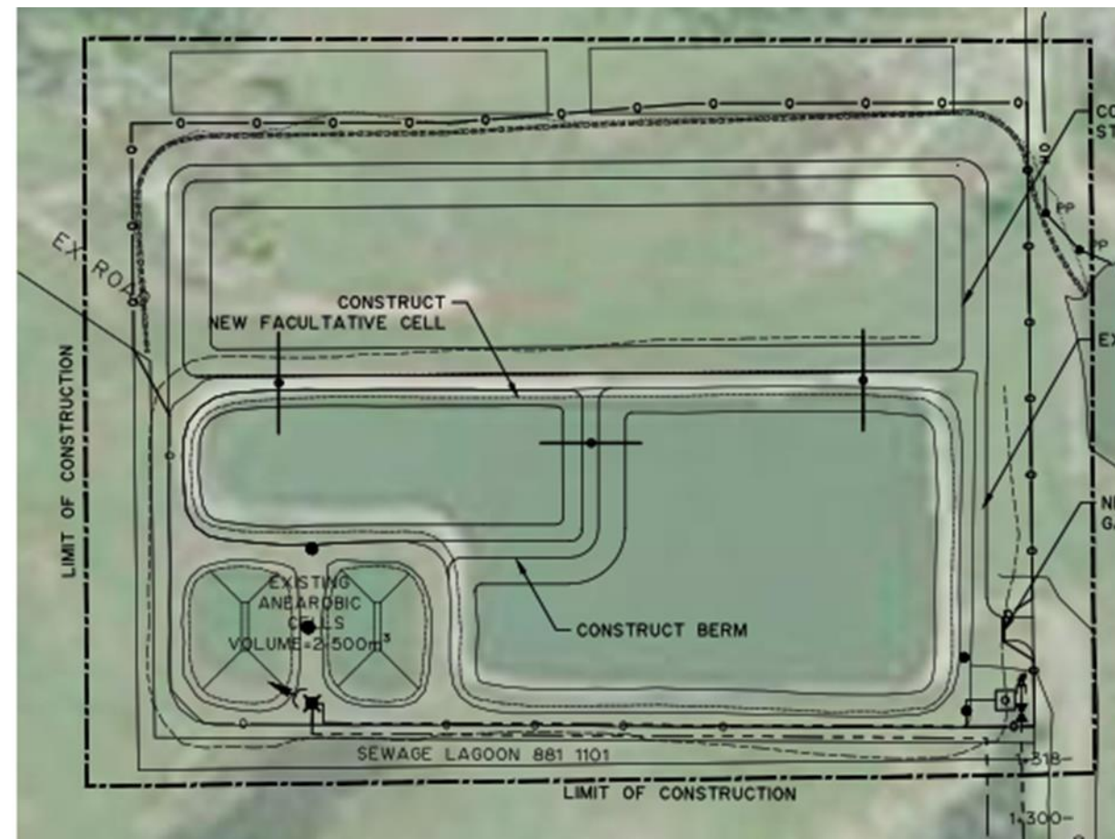
PROPOSED UPGRADED LAGOON TREATMENT SYSTEM
